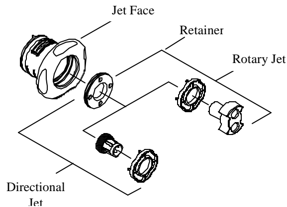
Figure 1: Obsolete Jet Heads with Jet Face
